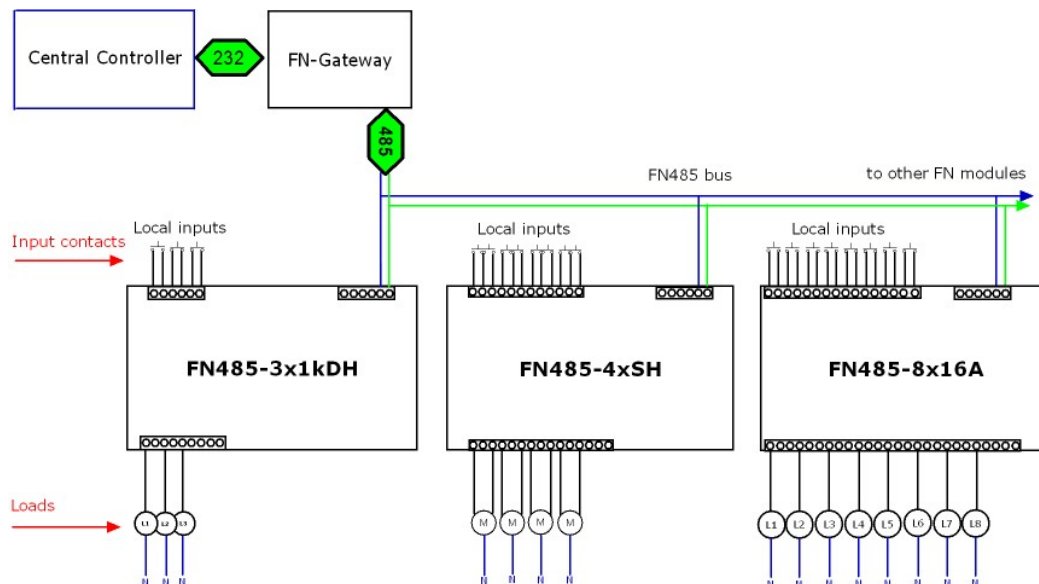
Figure 2. Connection diagram of an FN485 bus connected to a central controller via an FN Gateway
