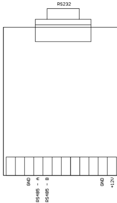
Figure 3. Terminal connections of the FN Gateway
